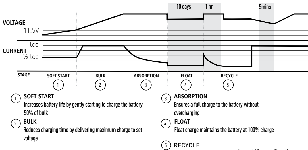
Figure 6 Charging Algorithm
