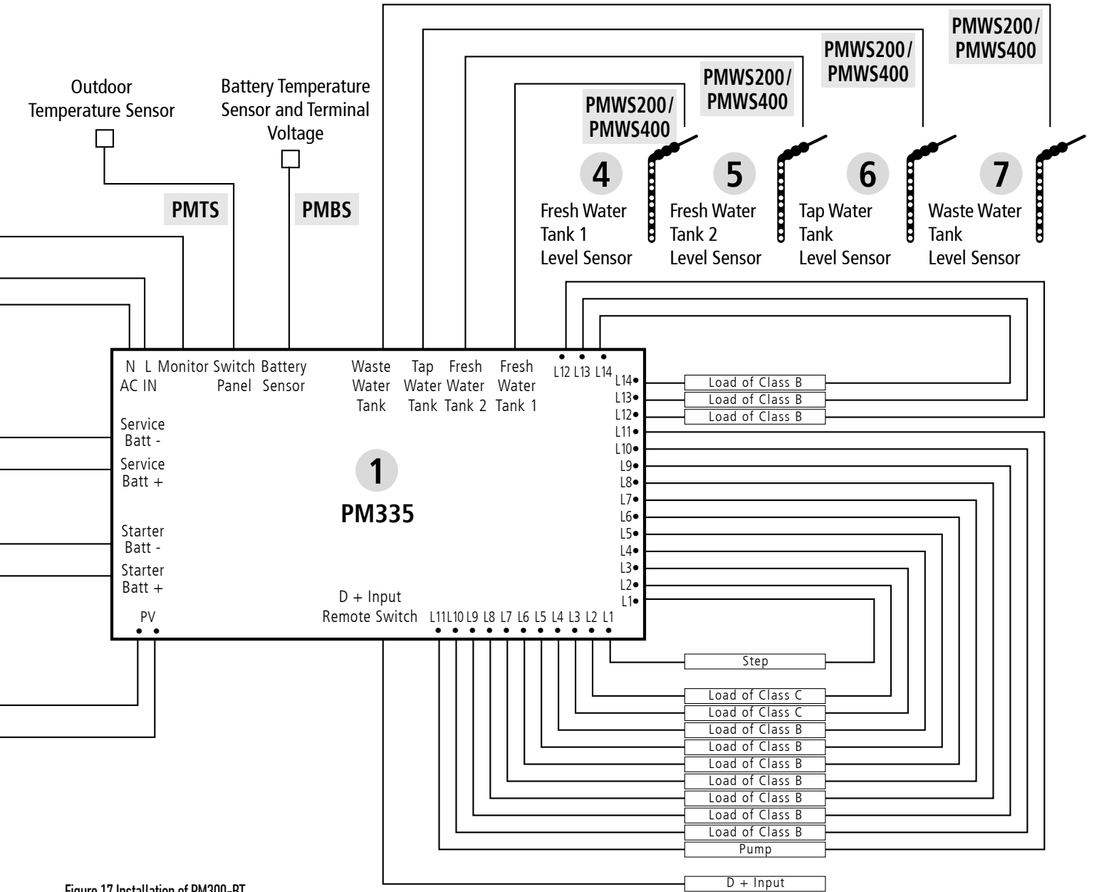
Figure 17 Installation of PM300-BT
