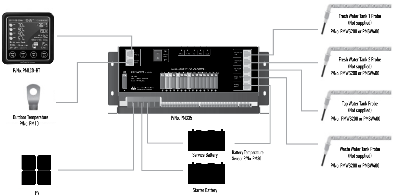
Figure 1 System Components for PM300-BT
