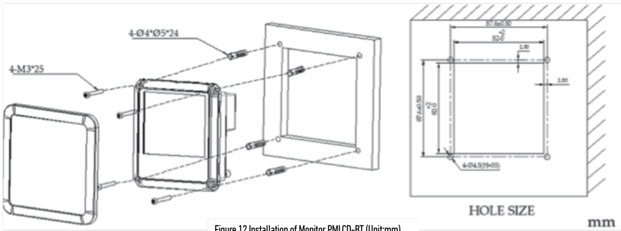
Figure 12 Installation of Monitor PMLCD-BT (Unit:mm)
